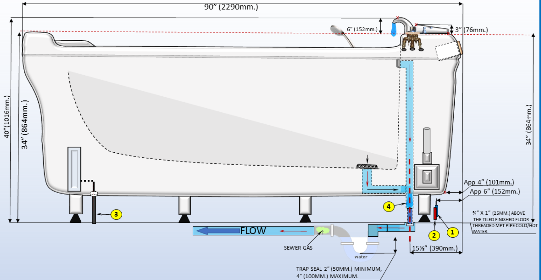
PLUMBING/ELECTRICAL DIAGRAM FOR RMS® PROFESSIONAL HYDROTHERAPY TUBS. JUMBO JUMBO LINE (ALL MODELS), UWM TUB TR-320MB-JL, L-105 JUMBO DE-LUXE.
